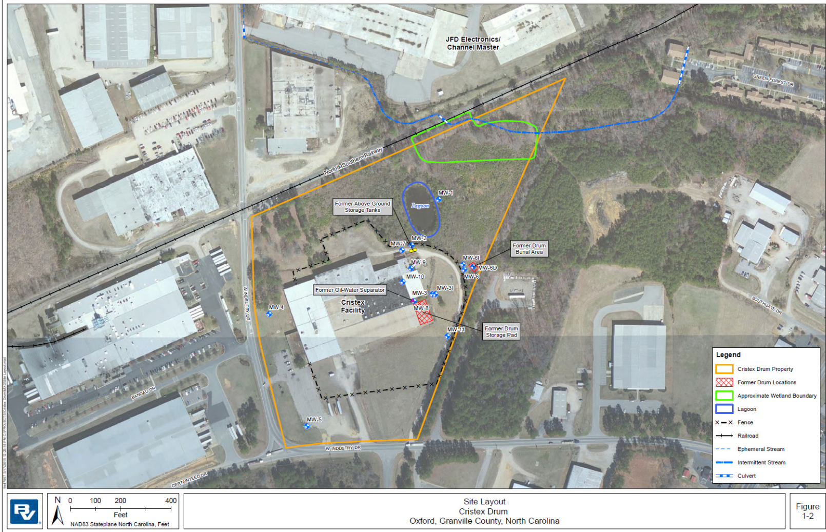
Figure 1. Cristex Drum NPL site layout. Oak Ridge Apartments are located N/NE of the Cristex facility on Green Forest Drive, visible in the upper right corner. Groundwater and surface water flows east.
